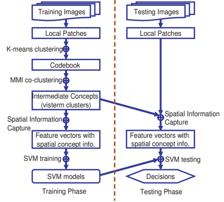
Figure 1. Work flow of the proposed scene classification framework.
