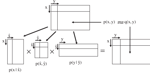
Figure 2. The graphical explanation of MMI co-clustering. The goal of MMI co-clustering is to find one clustering of X and Y which minimize the distance between the distribution matrix p(x, y) and q(x, y) .
