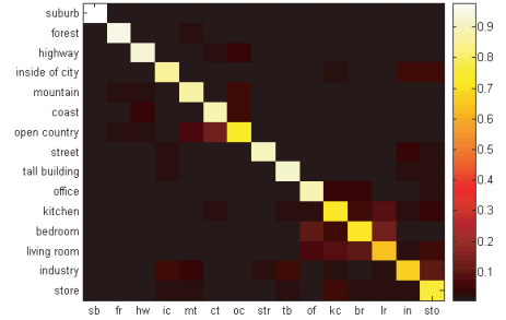
Figure 3. Confusion table for the SCC+BOC model. The average performance is 81.72%.
