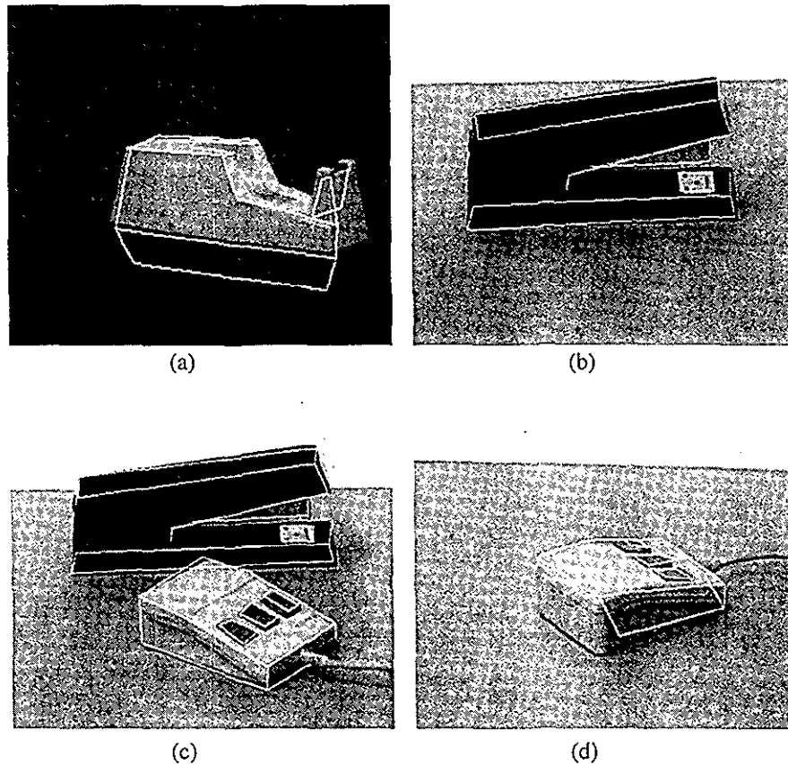
FIG. 11. Real scenes and recognition results.
