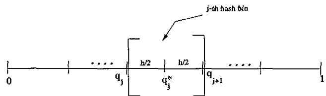
FIG. 8. Demonstration of the index-generation process.
