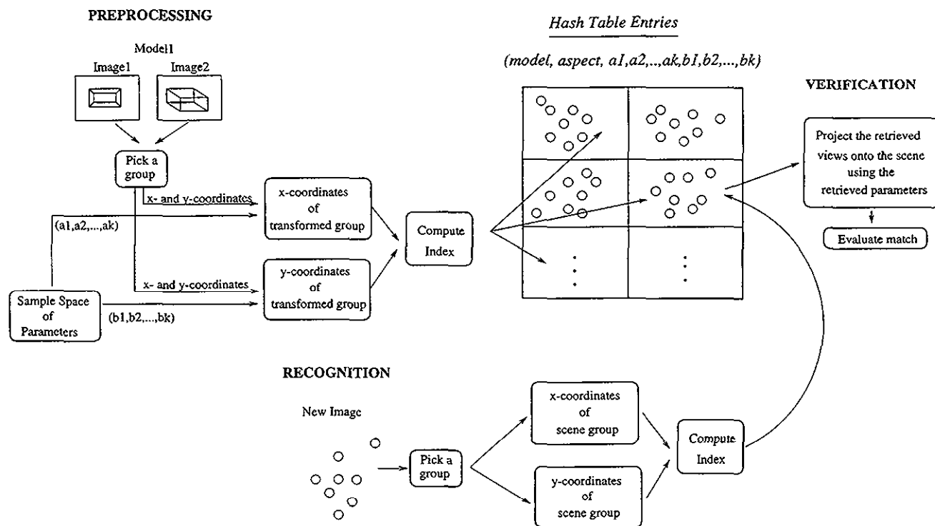
FIG. 1. A framework for indexing using algebraic functions of views.
