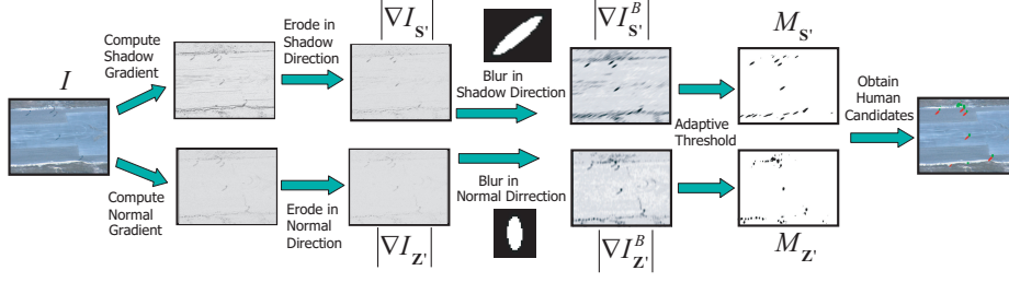
Fig. 3. This figure illustrates the pipeline of applying image constraints to obtain an initial set of human candidates.
