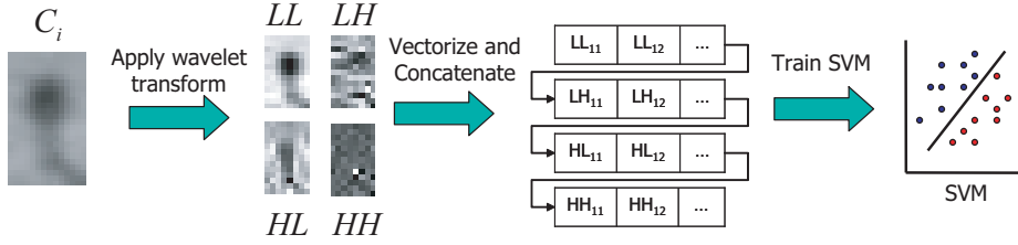
Fig. 6. Object candidate classification pipeline. Four wavelet filters (LL, LH, HL, HH) produce scaled version of original image, as well as gradient like features in horizontal vertical and diagonal directions. The resulting outputs are vectorized, normalized, and concatenated to form a feature vector. These feature vectors are classified using SVM.
