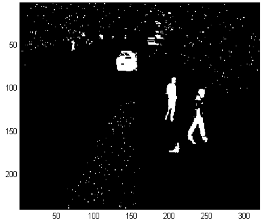
Single Gaussian Distribution
